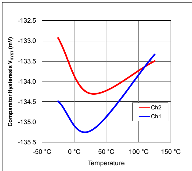
Figure 13: Comparator Hysteresis vs. Temperature
