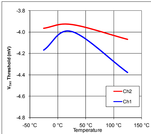
Figure 11: V_{TH1} vs. Temperature
