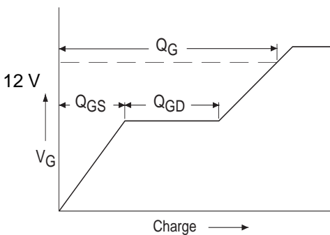
Fig30a. Basic Gate Charge Waveform
