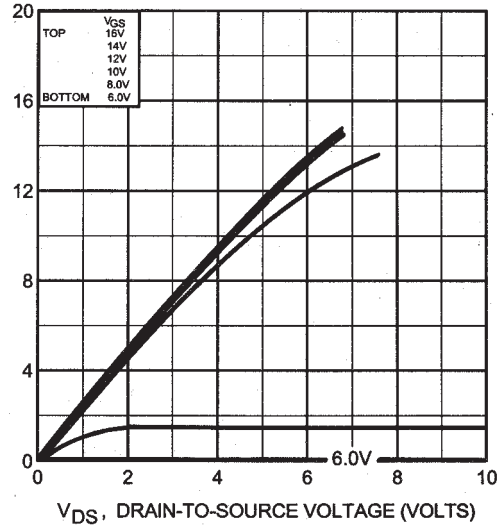
Fig 11. Typical Output Characteristics Post-Irradiation 100K Rads (Si)
